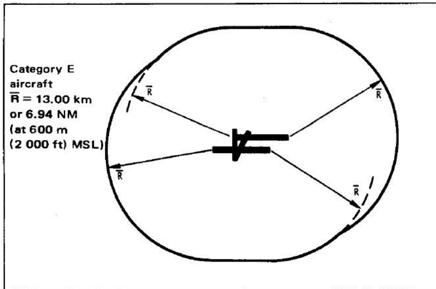
Figure III-8-1. Construction of visual manoeuvring (circling) area
