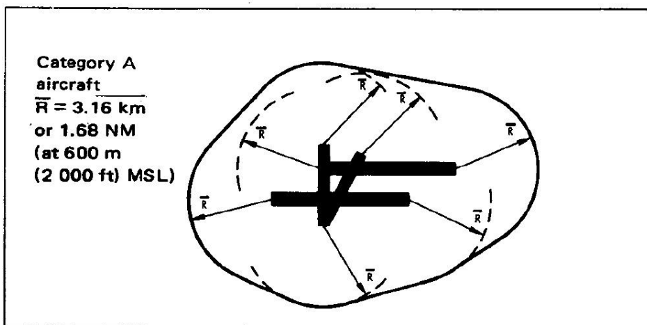
Figure III-8-2. Visual manoeuvring (circling) area
